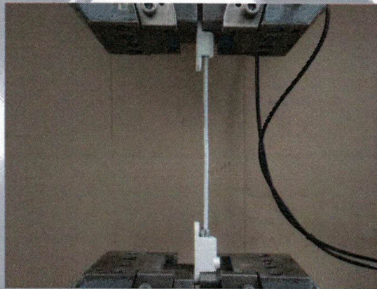
Photo 2 – Test setup
